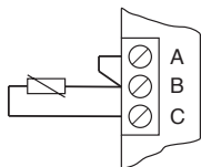
RTD/Thermistor (2-wire)
