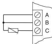
RTD/Thermistor (3-wire)
